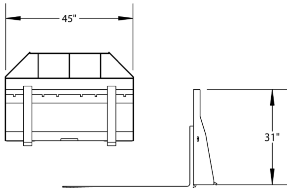
Compact Tractor Pallet Forks & Frame Specs
